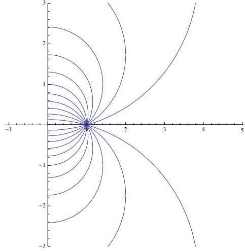
Figure 2: Field of a particle in hyperbolic motion, with b = 1 (naive).
