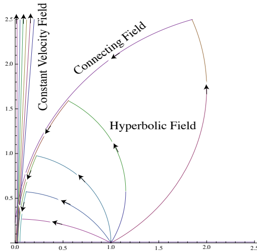
Figure 4: Truncated hyperbolic motion, for large \alpha , showing the “connecting” field.
