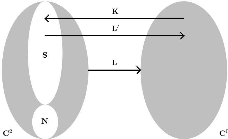
Differential/Integral Operators
