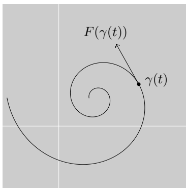
Integral Curve
