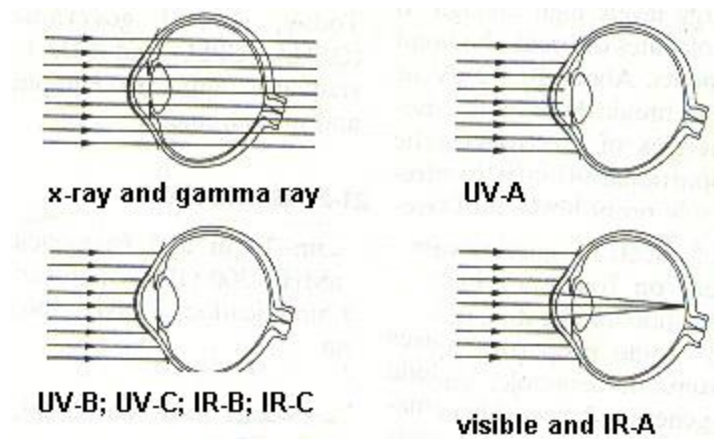
Figure Appx 4.1: Electromagnetic Radiation and the Eye
