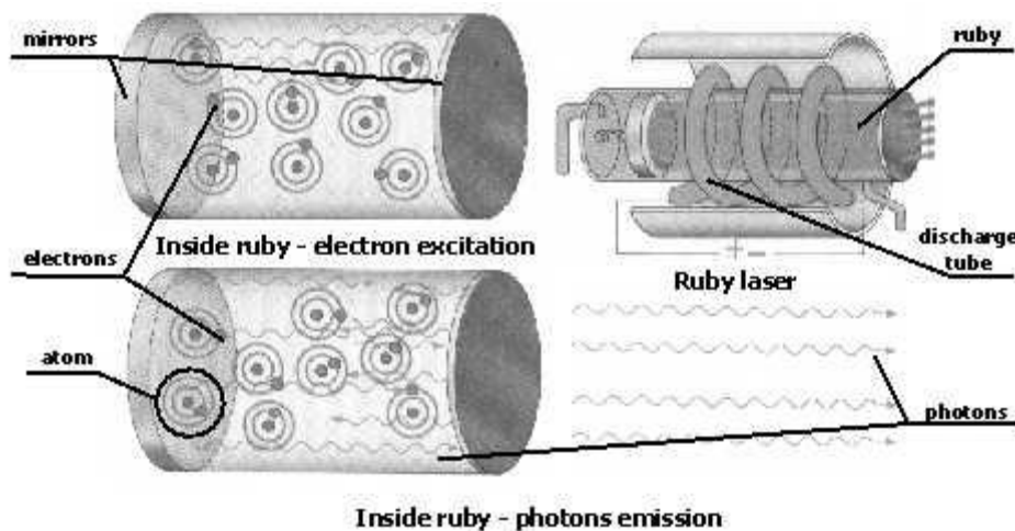
Figure Appx 2.1: Ruby Laser
